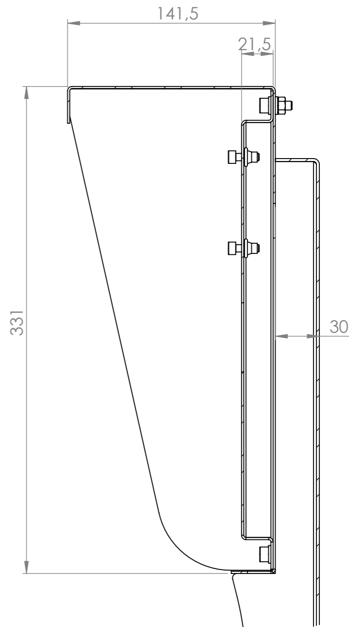
DETAIL B SCALE 2 : 5
